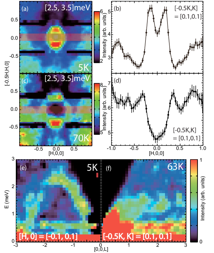
FIG. 3. (a) Low energy ( E = 3 \pm 0.5 meV) spin waves of \text{CrI}_3 in the [H, K] plane at T = 5 K. (b) A cut along the [H, 0] direction. (c) The same scan as (a) but at T = 1.14T_c . (d) The same cut as (b) at T = 1.14T_c . The red boxes in (a) and (c) show the integration range in (b) and (d), respectively, with L integrated from [-5, 5] . (e) Spin wave dispersion along the c axis at T = 5 K. (f) Identical scan at T = 1.03T_c . The data was collected using E_i = 8 meV [23].
