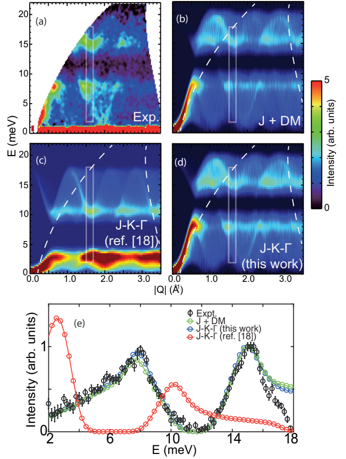
FIG. 5. (a) INS data of the \text{CrI}_3 powder at T = 5 K using E_i = 25 meV. (b)–(d) Powder-averaged spin-wave spectra calculated using the Heisenberg-DM [31], J - K - \Gamma Hamiltonian using parameters of Ref. [18], and new parameters ( J_1 = -0.17 \pm 0.05 meV, J_2 = -0.21 \pm 0.04 meV, K = -5.6 \pm 0.2 meV), respectively. The dashed lines mark the limits of the data in (a). (e) The black, green, red, and blue points/lines are the experimental data, Heisenberg-DM, J - K - \Gamma Hamiltonian calculations with parameters of [18], and the new parameters mentioned above, respectively. The scan directions are marked as solid boxes in (a)–(d).
