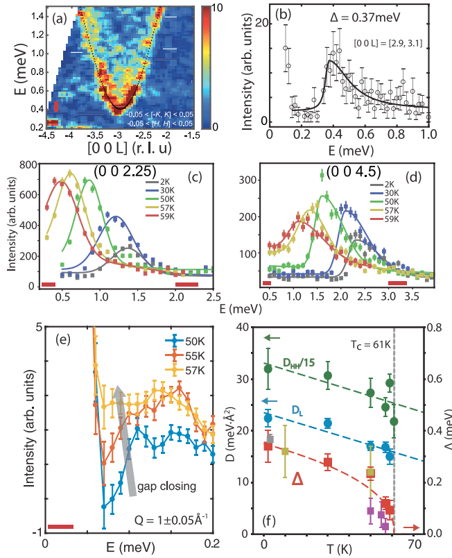
FIG. 2. (a) Images of spin waves near the \Gamma point. (b) An energy cut of the data at \mathbf{Q} = (0, 0, -3) . (c) Constant- \mathbf{Q} scans for \mathbf{Q} = (0, 0, 2.25) . (d) Similar scans at \mathbf{Q} = (0, 0, 4.5) . (e) Temperature dependence of the spin gap around the \Gamma point [23]. (f) Temperature dependence of the D_{HH}(T) (green dots), D_L(T) (blue dots), and \Delta(T) (Gray (LET), red (PANDA), yellow and purple (both Pelican) colored squares), where the dashed line is a fit to the power law equation. The green and blue dashed lines are guides to the eye.
