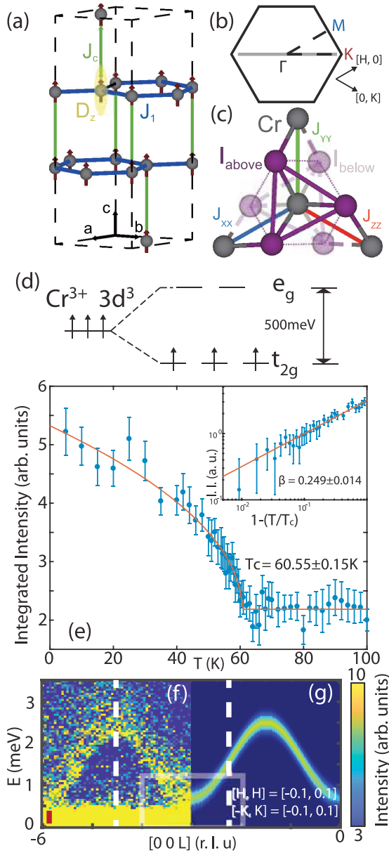
FIG. 1. (a) Crystal structure of \text{CrI}_3 , where the nearest neighbor magnetic exchange couplings within the Cr plane and along the c axis are J_1 and J_c , respectively. The D_z is the single-ion anisotropy. (b) Reciprocal space within the [H, K] plane, where \Gamma , K , M points are specified. The gray line indicates the \mathbf{Q} direction for constant-energy scans. (c) Real space picture of \text{CrI}_3 , where the nearest-neighbor I atoms form an octahedral environment with 3 I above (dark purple) and 3 I below (light purple) the Cr layer. The Cr-I-Cr path forms an angle close to 90 degrees [12,13]. The Kitaev interactions between \text{Cr}^{3+} atoms are marked as J_{xx} , J_{yy} , and J_{zz} [18]. (d) The CEF level of the I octahedra splits the d levels in the e_g and t_{2g} manifolds. (e) Magnetic order parameter at the (1, 1, 0) position. The inset is a log-log plot of the integrated magnetic peak intensity. Both red lines are power law fits with the same critical exponent \beta = 0.249 \pm 0.014 . (f) Spin-wave dispersion along the [0, 0, L] direction at T = 3 K obtained with E_i = 5.2 meV. (g) The Heisenberg model fit of the c -axis dispersion. The dashed lines in (f) and (g) indicate const- \mathbf{Q} scans in Figs. 2(c) and 2(d). Red bars in (f) and Figs. 2(a), 2(c), 2(d), 2(e), 3(a), and 4(a) are instrumental energy resolution [23].
